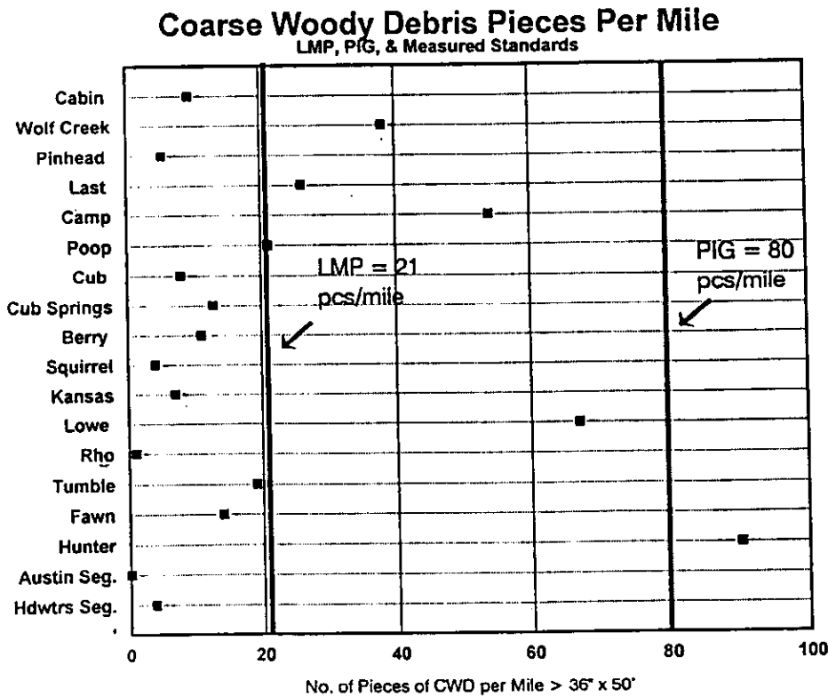
Figure 3-15. Average pieces of coarse woody debris (> 36 inches diameter and > 50 feet long) per mile for sampled streams by natural group with LMP and PIG numeric standards.
