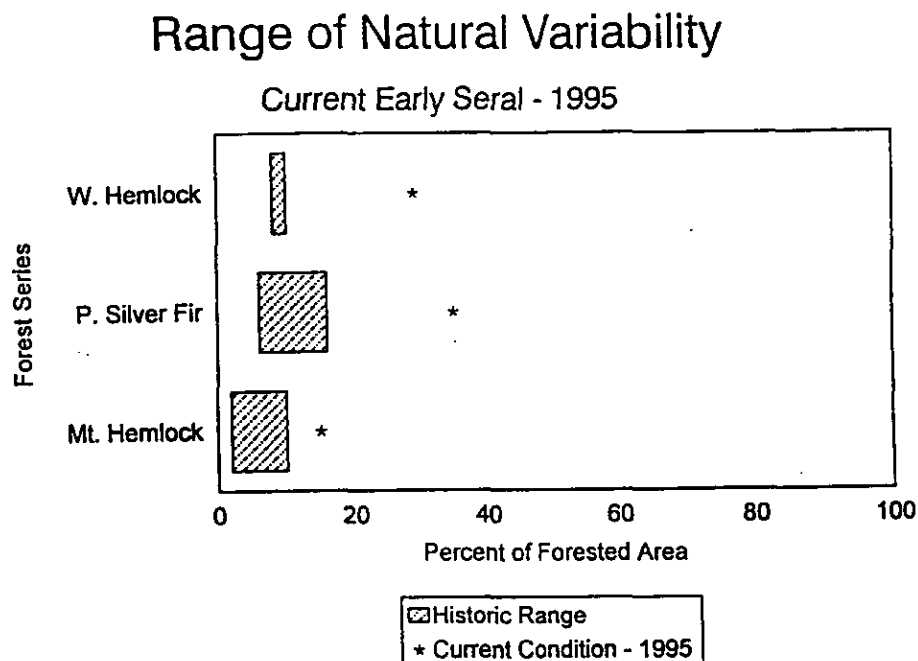
Figure 3-3. Current condition compared to historic range of amount of early seral vegetation. Values shown are percentage of the total area within each forest series.
