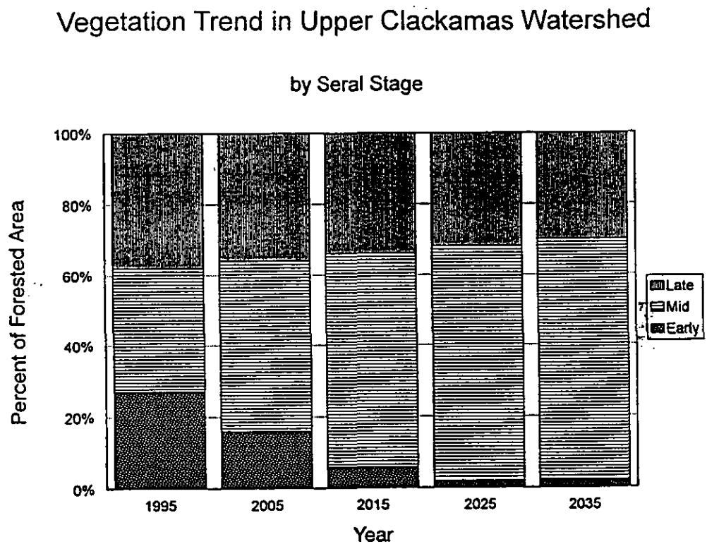
Figure 5-1. Vegetation trend in the Upper Clackamas watershed.
