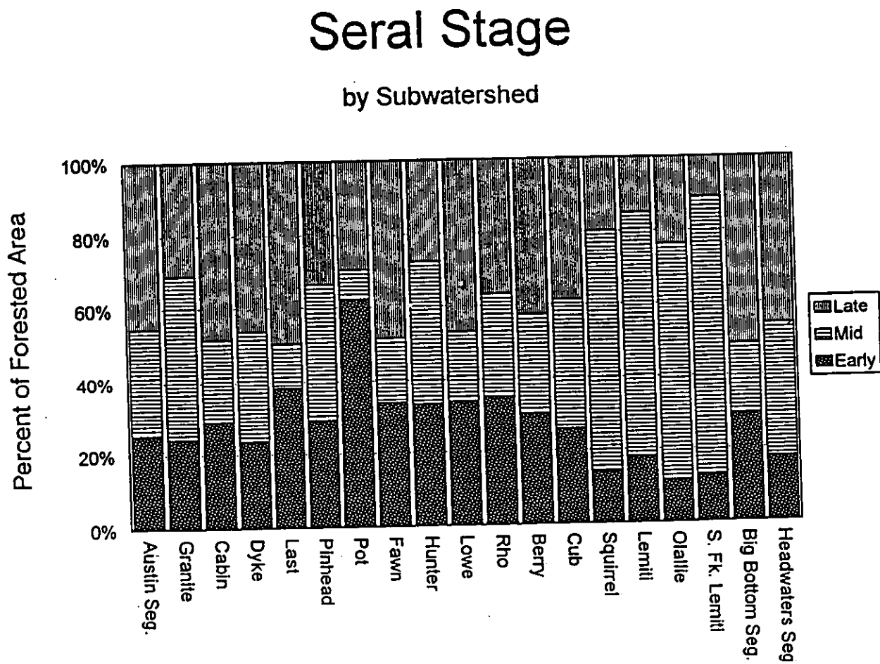
Figure 3-1. Seral stage by subwatershed. Values shown are percentage of each subwatershed in early, mid, and late seral stage.
